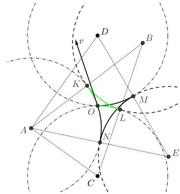
Fig. A.1. Feasible Reeds-Shepp's paths to change the heading at point O by \theta \in [0, \pi] and \pi + \theta , Path 1 and Path 2 , respectively.
