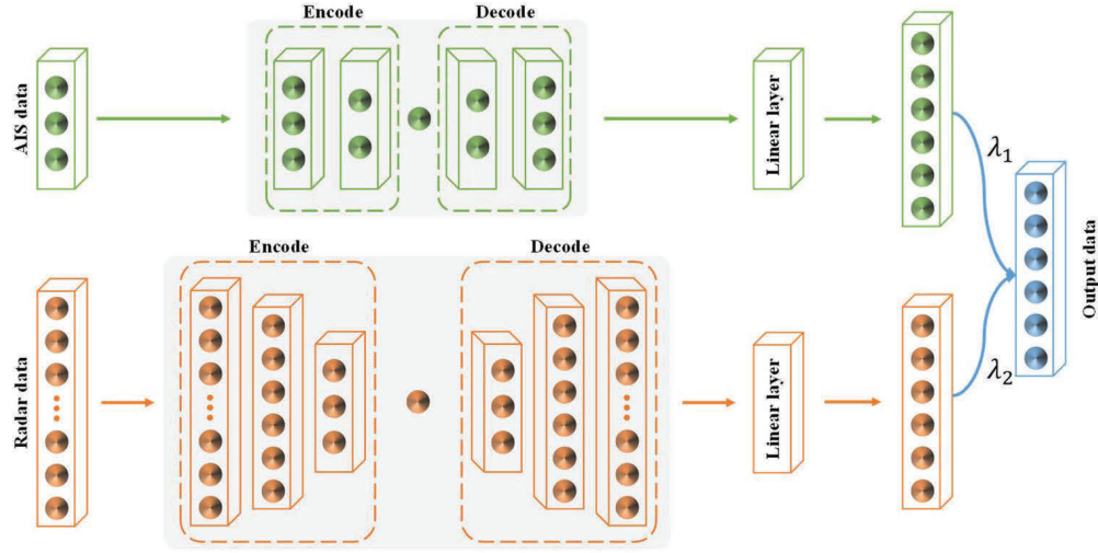
Fig. 6. Principle of SAE.
