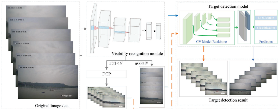
Fig. 7. Proposed target detection process.
