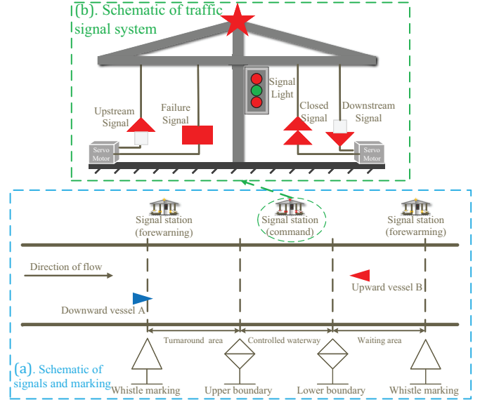
Fig. 1. Schematic of signals and markings in controlled waterway.
