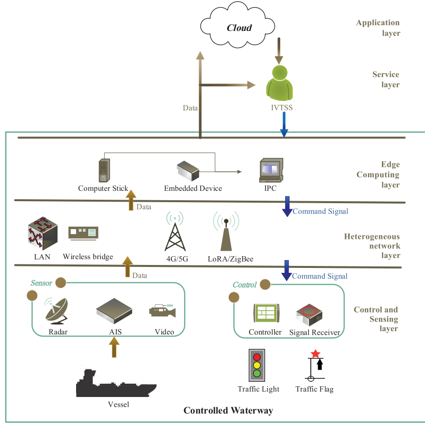
Fig. 3. Overall architecture of edge-centric IoT serving UR-IVTSS.
