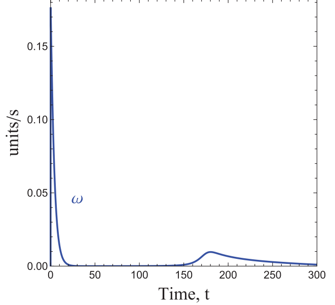
(f) Angular velocity graph
