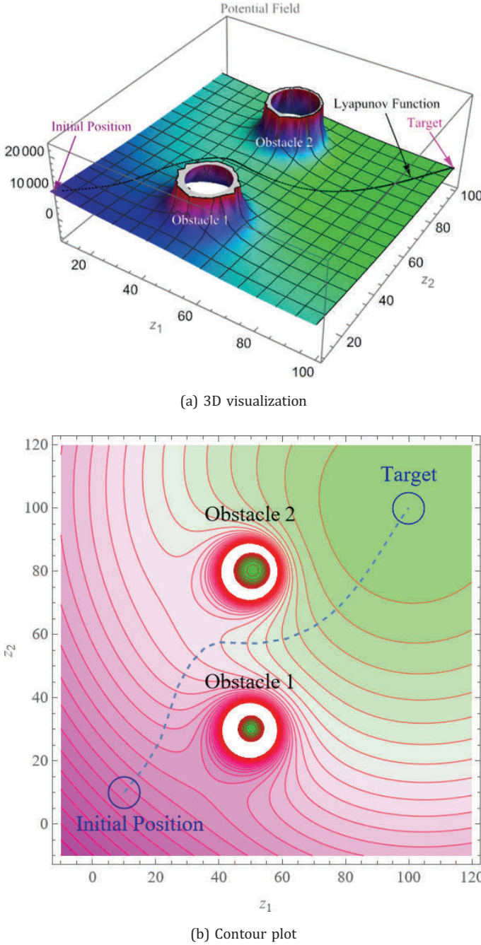
Fig. 1. An illustration of LbCS in a workspace comprising two obstacles.
