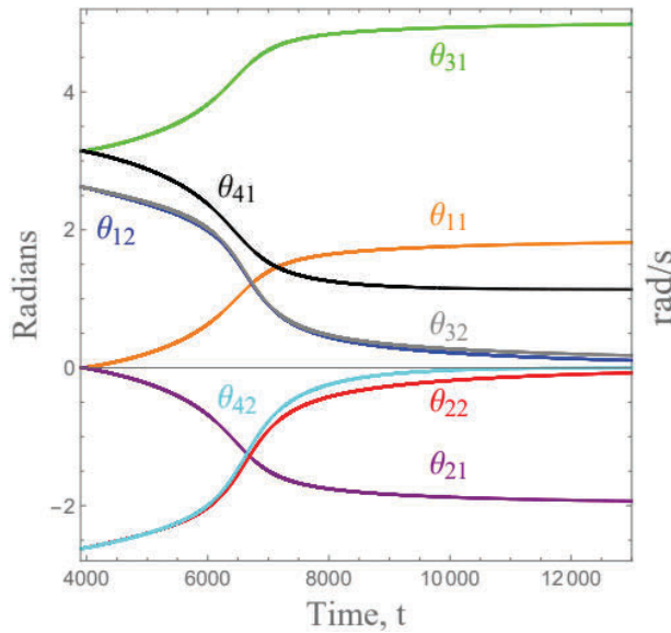
(c) Revolute link orientations
