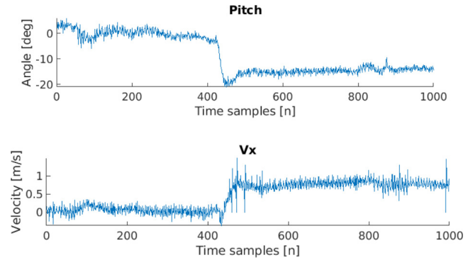
Fig. 6. Pitch step input of 12^\circ and its corresponding transient response in V_x .
