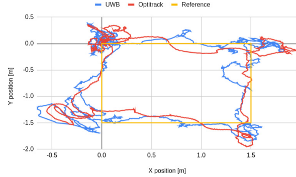
(b) Paths obtained with Kalman filter
