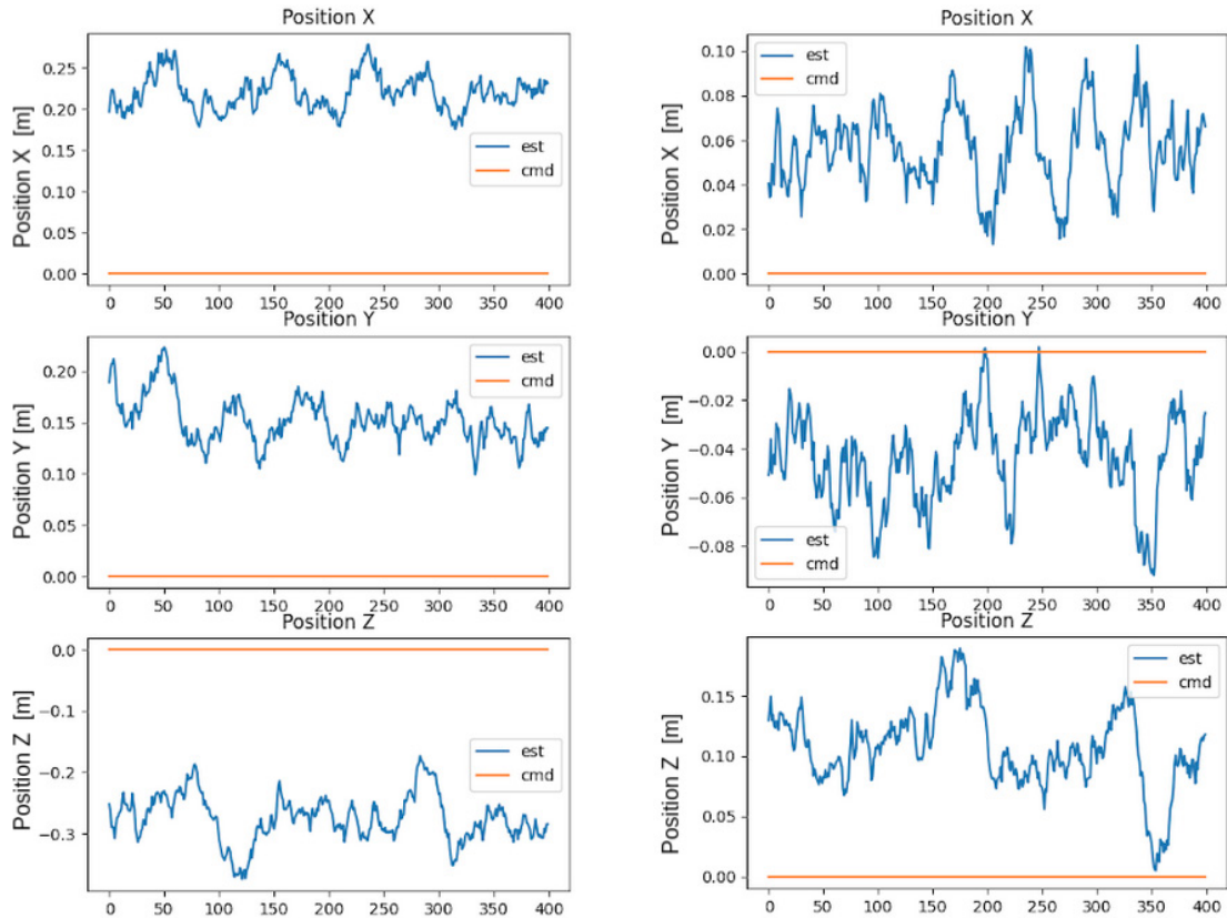
Fig. 4. Effects in position estimation before using variable sensor noise (left) and after implementing it (right).
