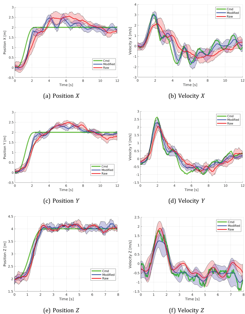
Fig. 13. Transient responses on position and velocity with a step input of amplitude 2.
