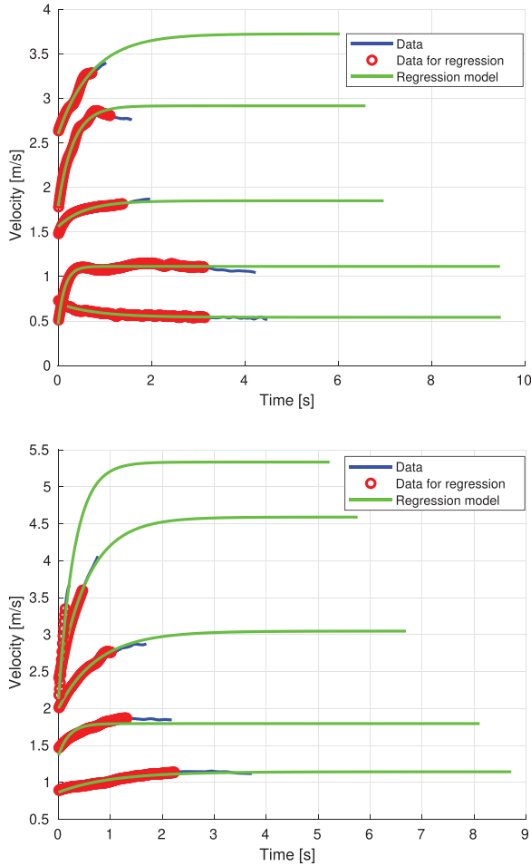
Fig. 8. Extrapolation models for pitch (top) and roll (bottom) at different velocities.
