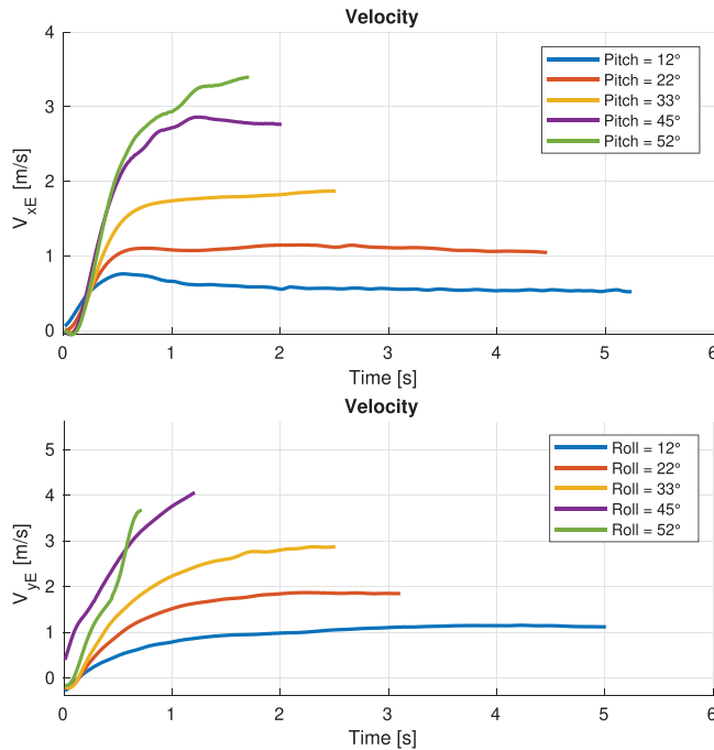
Fig. 7. Velocities attained at different pitch and roll step inputs.
