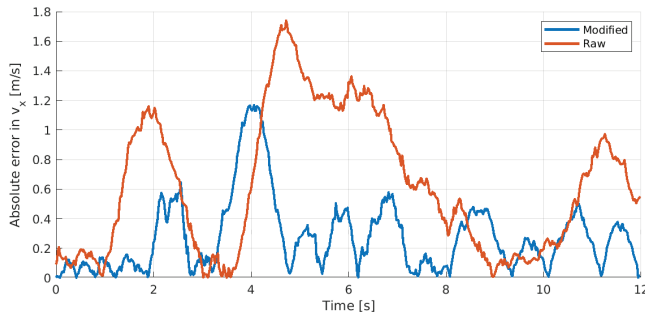
(a) Absolute error in Velocity X
