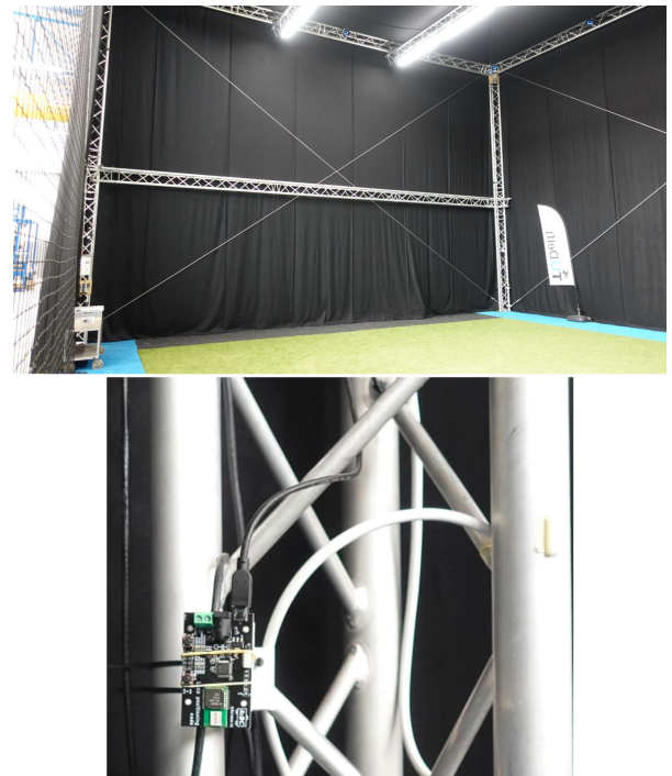
Fig. 1. Cyberzoo structure where the UWB anchors are placed (top) and detail of UWB anchor mounted on the structure (bottom).
