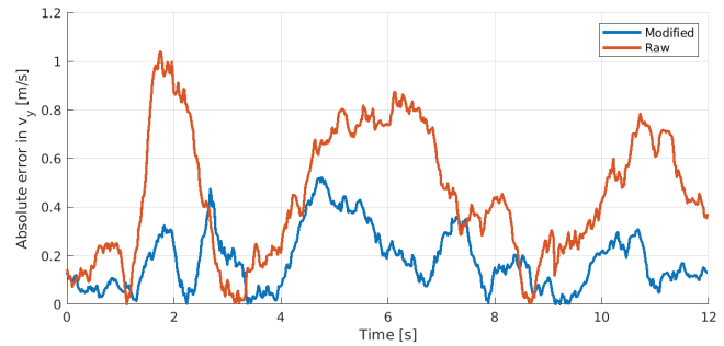
(b) Absolute error in Velocity Y
