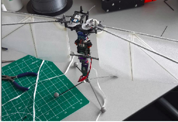
Fig. 2. Flapper drone with IR markers and UWB sensor.
