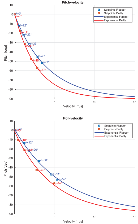
Fig. 9. Pitch/velocity (top) and roll/velocity (bottom) models obtained from extrapolated data.
