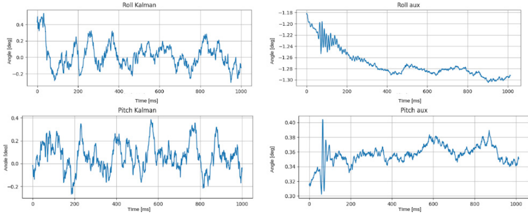
Fig. 3. Roll and pitch estimation of the drone at static position using Kalman (left) and complementary (right) filter.
