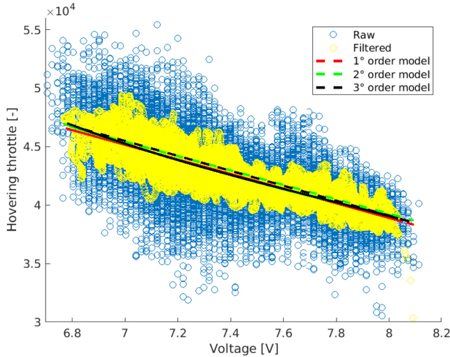
Fig. 10. Throttle and voltage mapping with tendency lines for different regression models.
