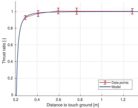
Fig. 12. Thrust ratio for each height.
