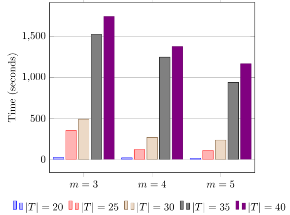
Fig. 5. Average time taken to compute the optimal solution for the formulation \mathcal{F}_2 .
