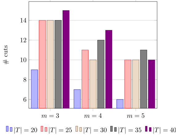
Fig. 6. Average number of violated constraints (7) identified by the branch-and-cut algorithm for the formulation \mathcal{F}_2 .
