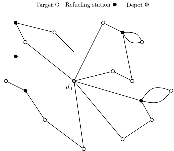
Fig. 2. A feasible solution to the FCMVRP. The solution is for a 4-vehicle problem. d_0 denotes the depot where all the vehicles are stationed initially. Note that a refueling station can be visited any number of times for refueling while some refueling stations may not be visited at all.
