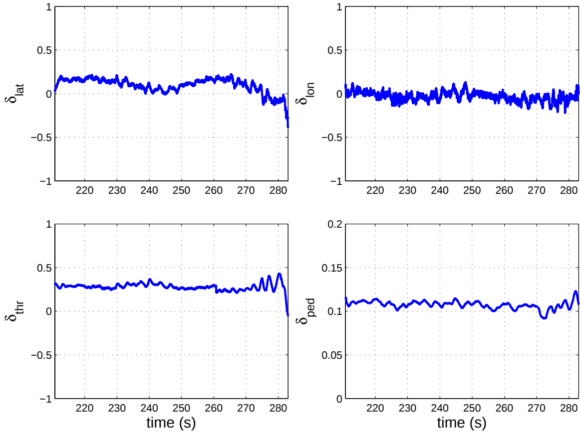
Fig. 33. Flight result: trajectory tracking — control effort.
