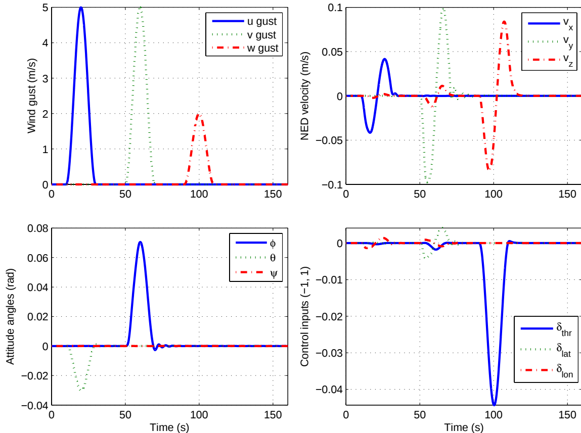
Fig. 31. Simulation results of the wind gust attenuation of the closed-loop system.
