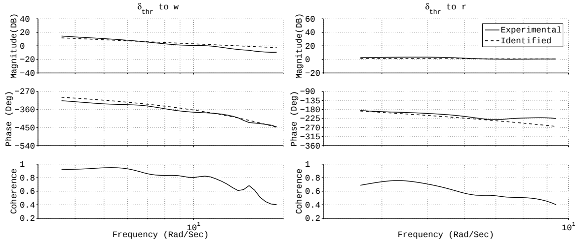
Fig. 24. System identification from \delta_{thr} to w and r .
