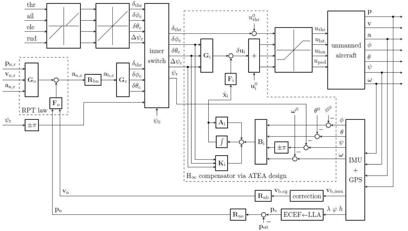
Fig. 28. Outer- and inner-loop control laws based on RPT and H_\infty approach via the ATEA design method.
