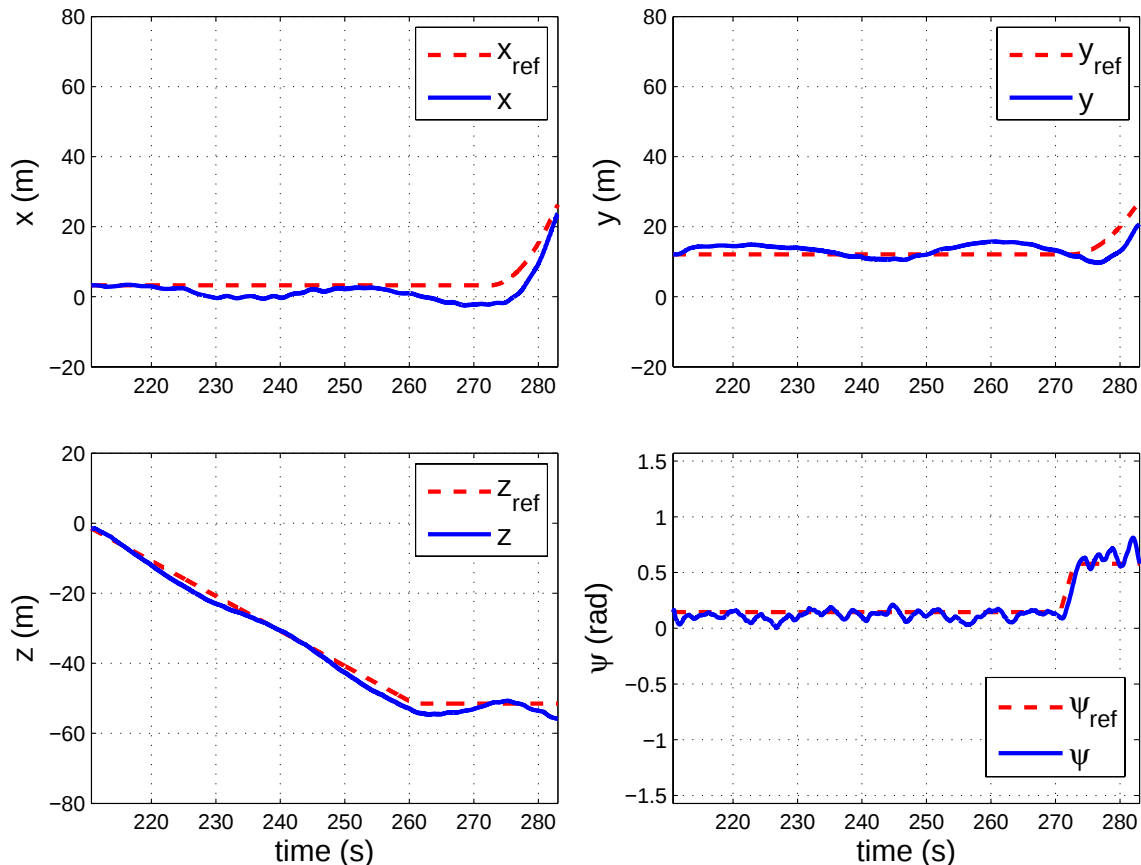
Fig. 32. Flight result: trajectory tracking — position and heading.
