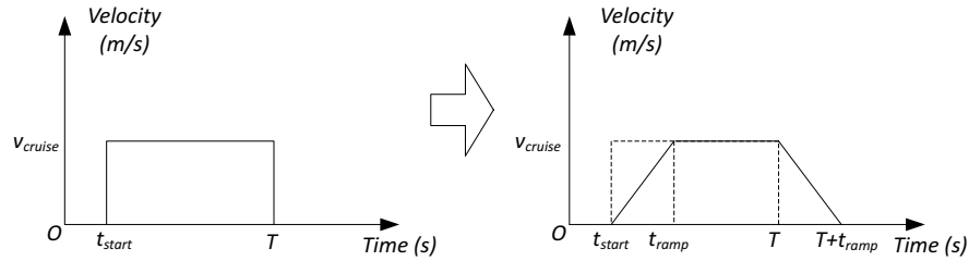
Fig. 29. Illustration of the velocity reference generation.
