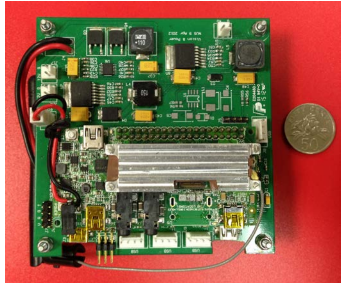
Fig. 12. The vision hub.
