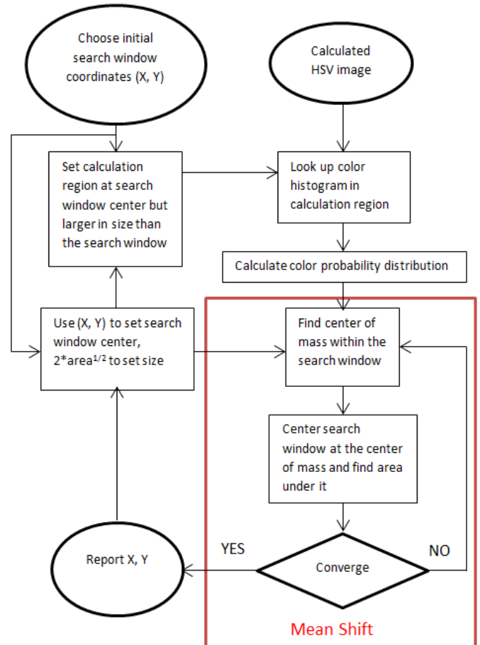
Fig. 39. The flowchart of the CAMSHIFT algorithm.
