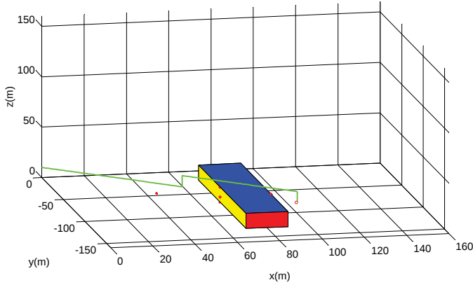
Fig. 38. (Color online) Simulation result for obstacle avoidance.
