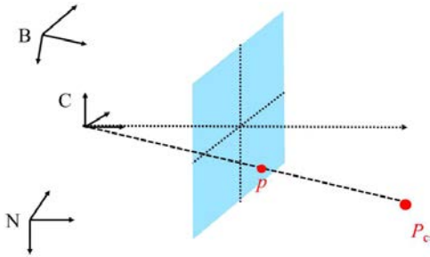
Fig. 34. Reference frames involved in depth estimation. N: NED frame, B: body frame, C: camera frame.
