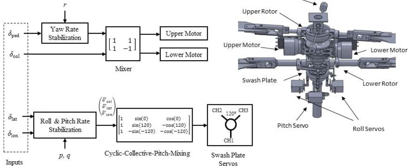
Fig. 10. Operating principle of GremLion.
