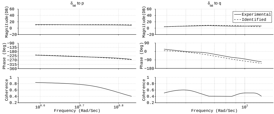
Fig. 25. System identification from \delta_{lat} to p and q .
