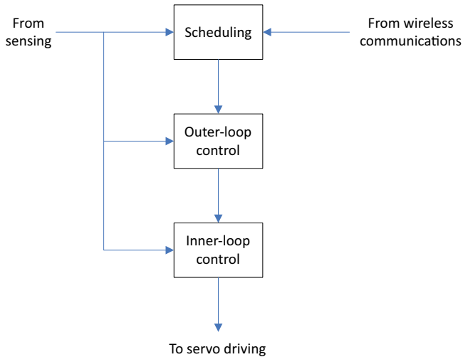
Fig. 17. Flight control description.
