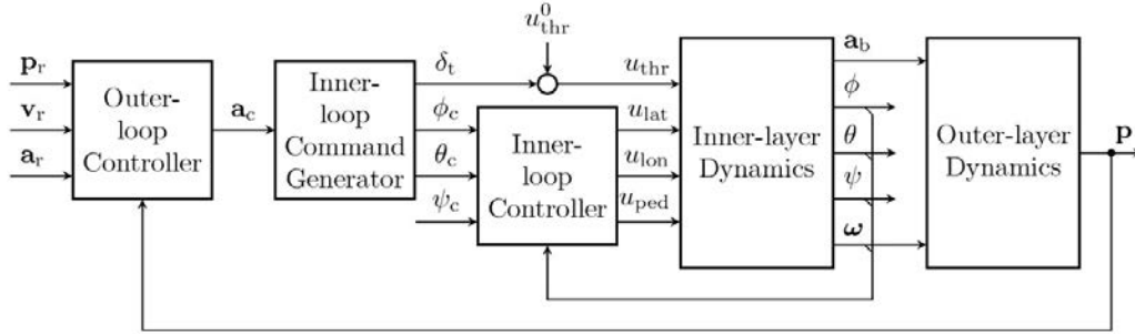
Fig. 27. Dual-loop structure of flight control system.
