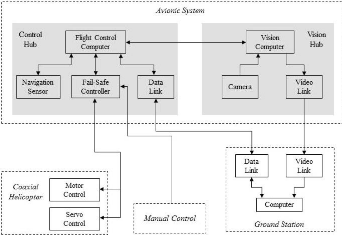
Fig. 6. Hardware configuration of GremLion.
