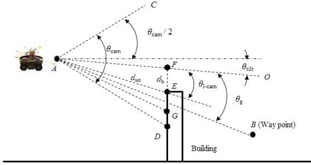
Fig. 37. Geometry for obstacle avoidance.
