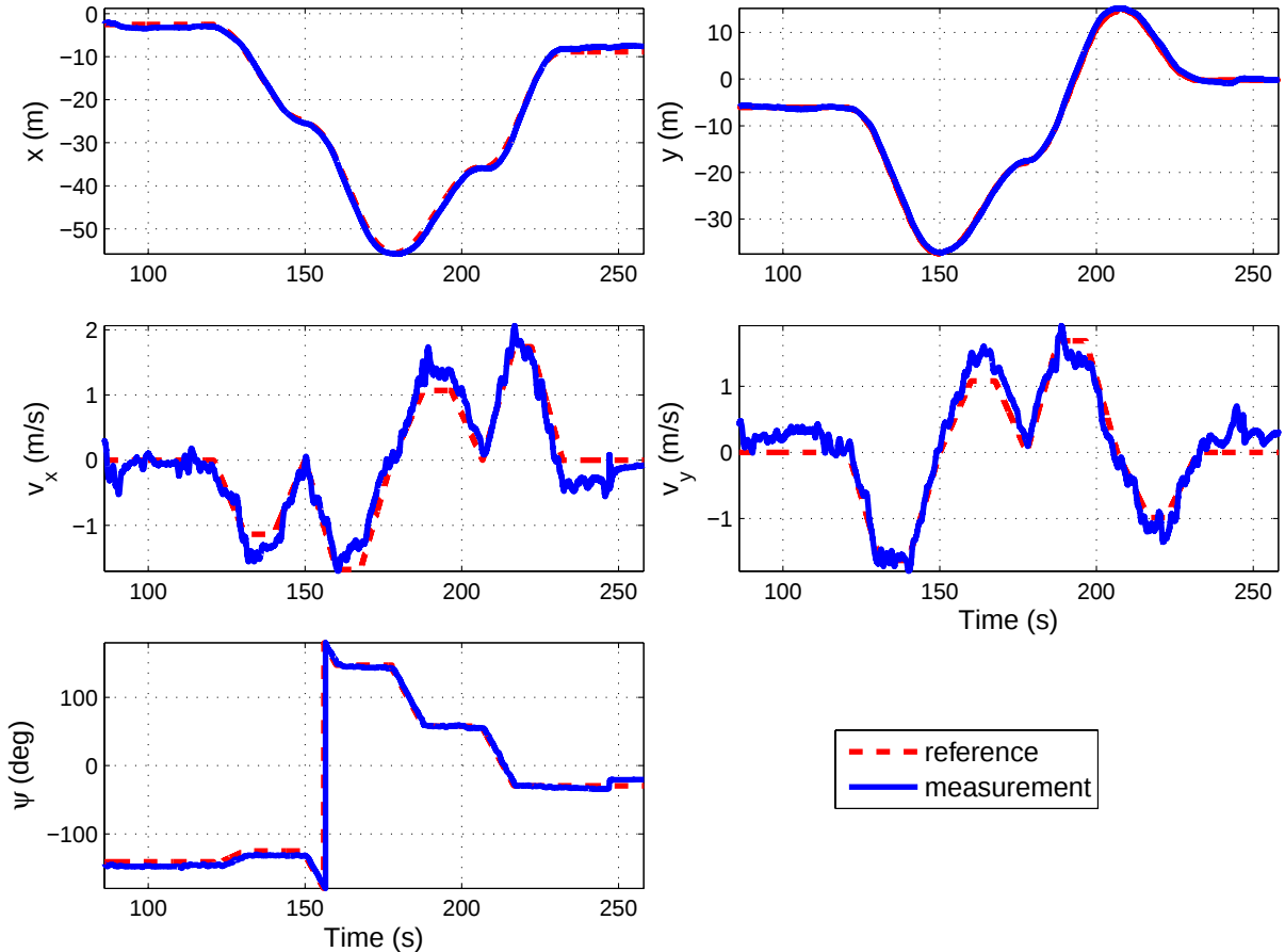
Fig. 30. Experimental results of the reference generation in flight.
