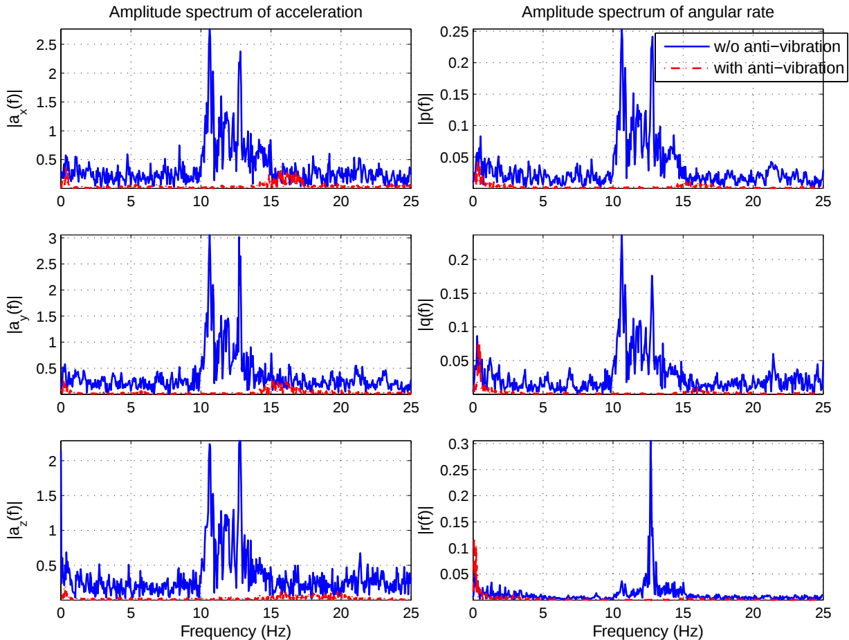
Fig. 13. Comparison of frequency response of the acceleration and angular rate with anti-vibration solutions.
