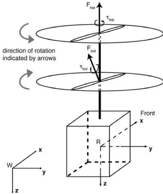
Fig. 9. The coaxial structure.
