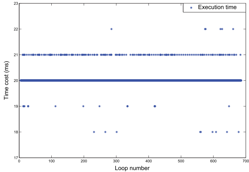
Fig. 20. Time intervals between each loop.
