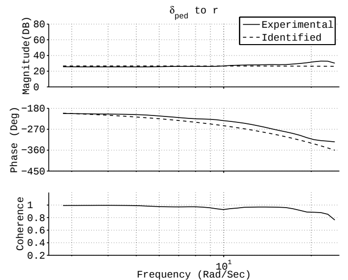
Fig. 23. System identification from \delta_{rud} to r .
