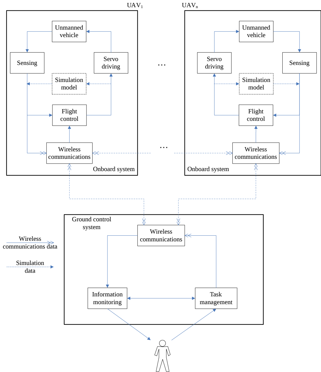
Fig. 15. Framework of UAV systems.
