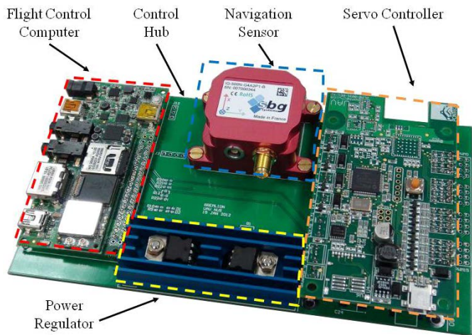
Fig. 11. Control Hub with all the modules.
