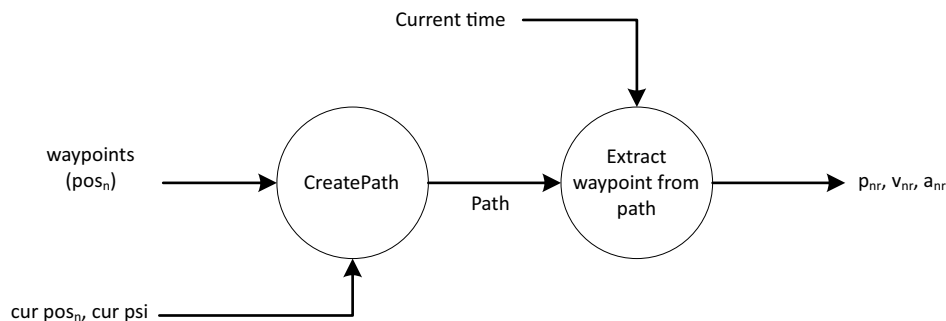
Fig. 18. Data flow diagram of autonomous reference generation.
