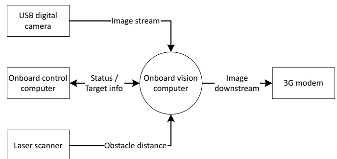
Fig. 21. UAV onboard vision software system.
