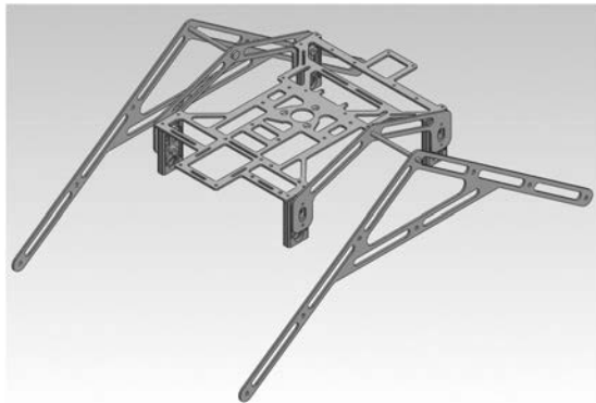
Fig. 14. Landing skid design.
