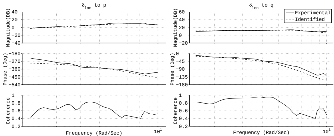
Fig. 26. System identification from \delta_{lon} to p and q .
