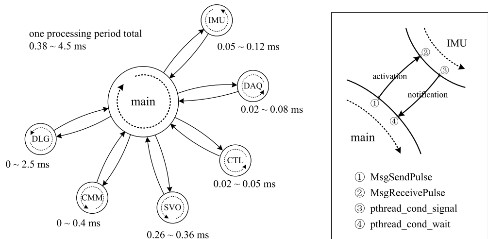
Fig. 19. Task management illustration diagram.
