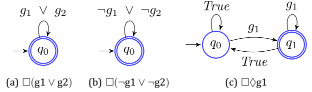
Fig. 5. Nondeterministic Buchi automata that recognize the desired properties of the traffic light system in Example 3.5. An arrow without a source points to an initial state. Accepting states are drawn with a double circle.
