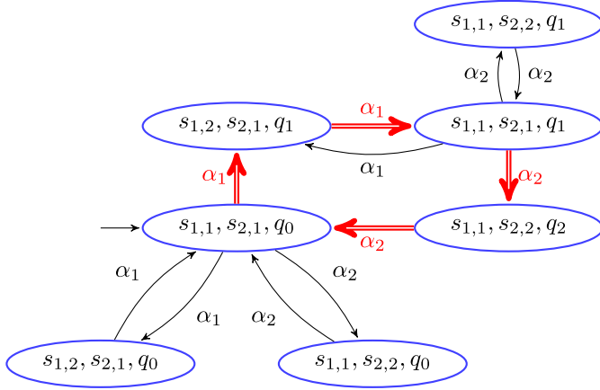
Fig. 13. (Color online) The product transition system TS_p = (T_1 \parallel T_2) \otimes \mathcal{A}_\varphi , showing only reachable states. An accepting path is highlighted by double (red) arrows.
