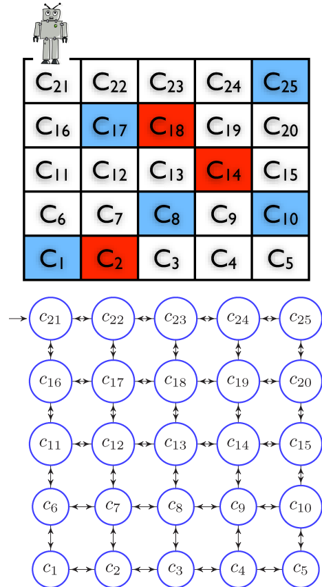
Fig. 7. (Top) The robot motion planning problem in Example 4.2 with the grid-based world model. (Bottom) The finite transition system that models the dynamics of the robot.
