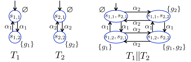
Fig. 3. The transition systems representing the models of traffic lights in Example 3.3.
