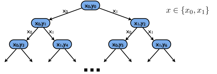
Fig. 14. A satisfying tree representing a control protocol for nondeterministic systems. The state of the system is a tuple (x, y) where x \in \{x_0, x_1\} represents the nondeterministic choice of the environment behavior whereas y \in \{y_0, y_1, \dots\} represents the state over which the system has control.
