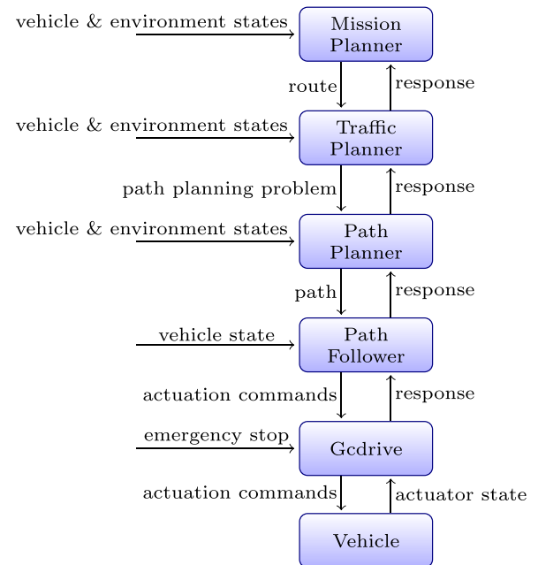
Fig. 1. Top. Alice, Team Caltech’s entry in the 2007 DARPA Urban Challenge. Bottom. Alice’s navigation protocol stack that reactively determines the motion of the vehicle based on the current state of its environment (as perceived by the sensing and estimation subsystems).
