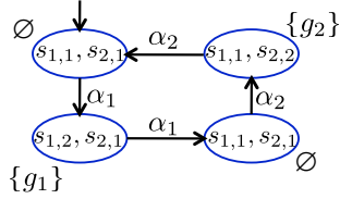
Fig. 6. (T_1 \parallel T_2)^C , the transition systems induced by applying C defined in Example 3.11 on the traffic light system T_1 \parallel T_2 .
