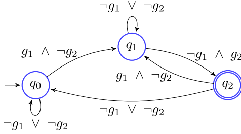
Fig. 12. Nondeterministic Buchi automata \mathcal{A}_\varphi that recognize \varphi = \Box(\neg g_1 \vee \neg g_2) \wedge \Box\Diamond g_1 \wedge \Box\Diamond g_2 . Accepted states are drawn with a double circle.
