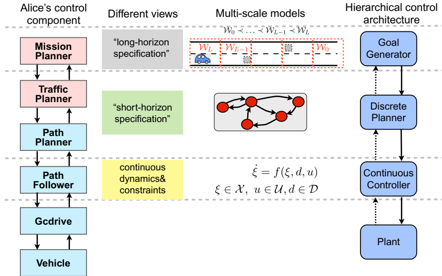
Fig. 18. The hierarchical control structure with the receding horizon implementation, showing the similarity with the navigation protocol stack implemented on Alice. The goal generator has similar functionality as Mission Planner. It determines a sequence of intermediate goals for the discrete planner such that the original “long-horizon” specification is satisfied. Its computation relies on the graph \mathbb{G} that encodes the partially ordered set (\{\mathcal{W}_0, \dots, \mathcal{W}_M\}, \prec_\varphi) . The discrete planner has similar functionality as the composition of Traffic Planner and Path Planner. It computes a discrete plan for the system such that the short-horizon specification in (12) with the next intermediate goal computed by the goal generator is satisfied based on a finite, abstract model of the physical system. Finally, the continuous controller deals with the continuous dynamics and constraints to ensure that the physical system follows the plan computed by the discrete planner. This functionality is similar to that of Path Follower in Alice.
