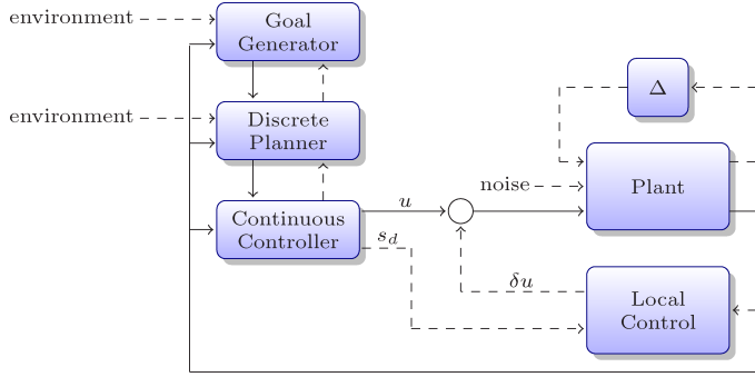
Fig. 17. The hierarchical control structure with the goal generator.
