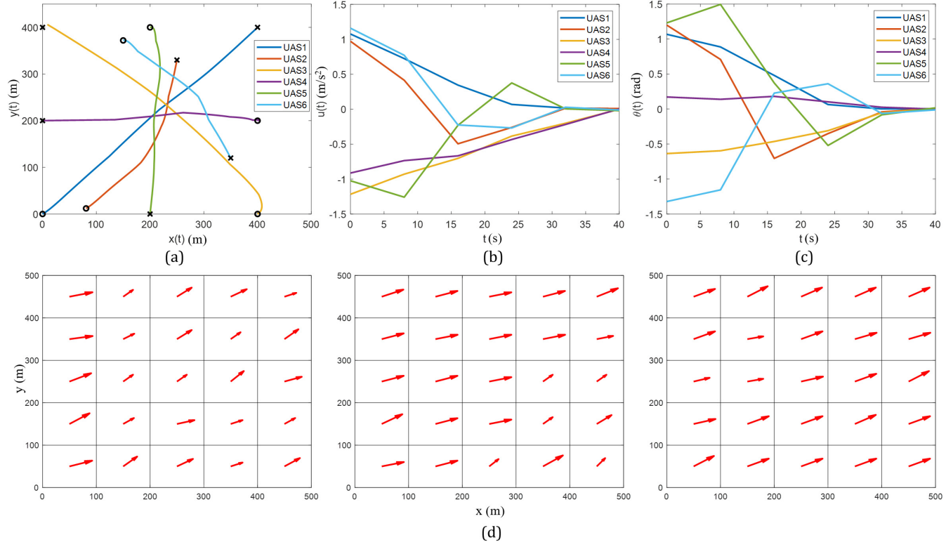
Fig. 9. The optimal 6 UASs trajectory solution for s_{C1} . (a) The trajectories of the 6 UASs. (b) The thrusts. (c) The angles of the thrusts. (d) The sample snapshots of s_{C1} at t = 5 s, t = 22 s, and t = 37 s.
