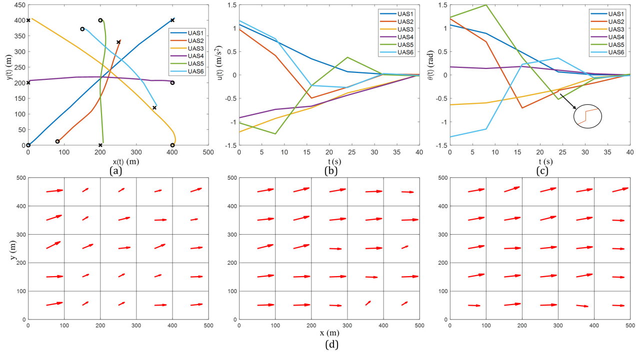
Fig. 10. The optimal 6 UASs trajectory solution for s_{C2} . (a) The trajectories of the 6 UASs. (b) The thrusts. (c) The angles of the thrusts. (d) The sample snapshots of s_{C2} at t = 5 s, t = 22 s, and t = 37 s.
