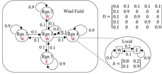
Fig. 2. A simple illustrative example of an influence model with five regions and two wind statuses “W” and “E”.
