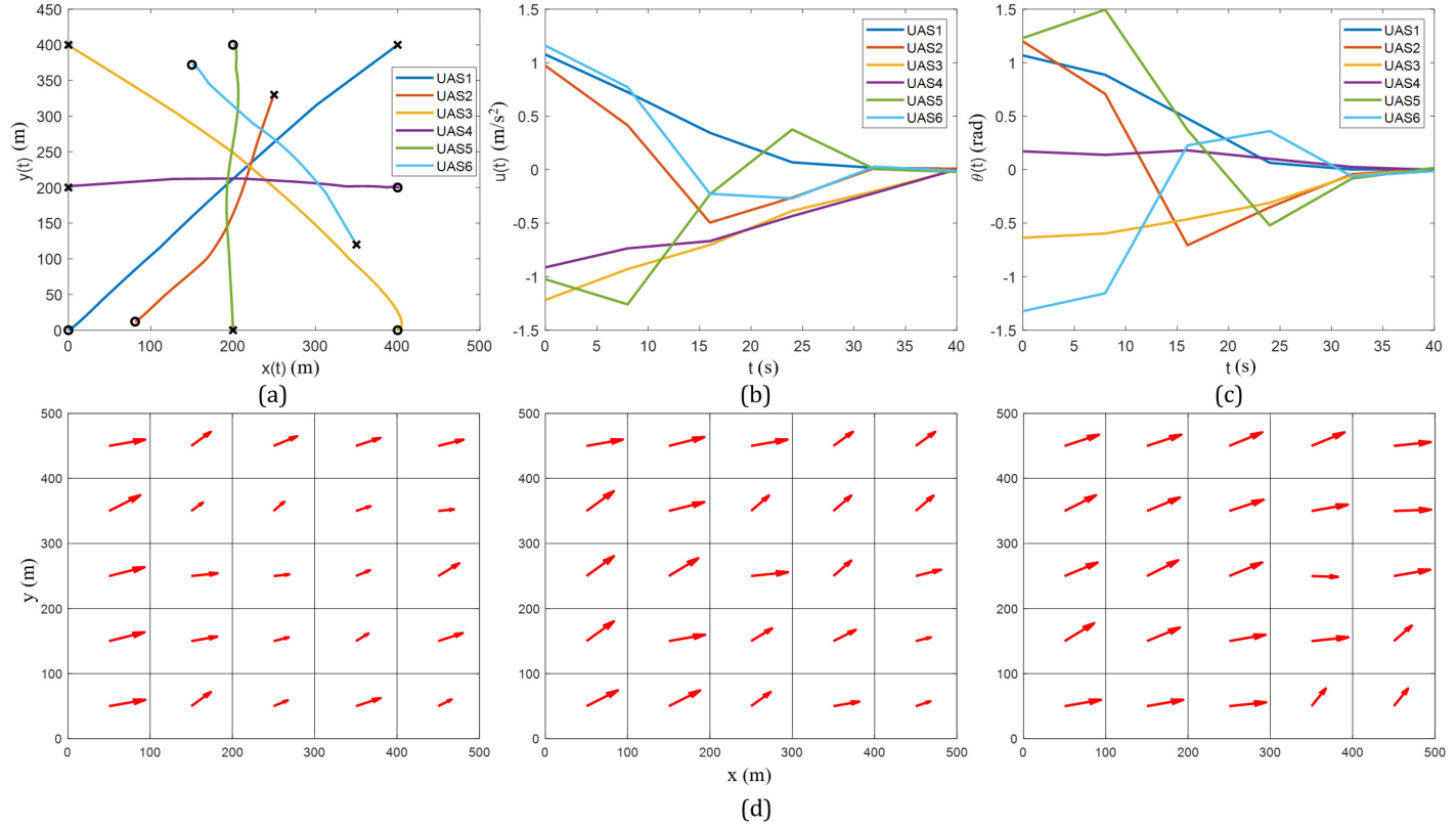
Fig. 8. An example for the optimal 6 UASs trajectory solution. (a) The trajectories of the 6 UASs. “Circle” denotes the starting point and “X” denotes the destination. (b) The thrusts. (c) The angles of the thrusts. (d) The sample snapshots of the spatiotemporal wind scenario at t = 5 s, t = 22 s, and t = 37 s.
