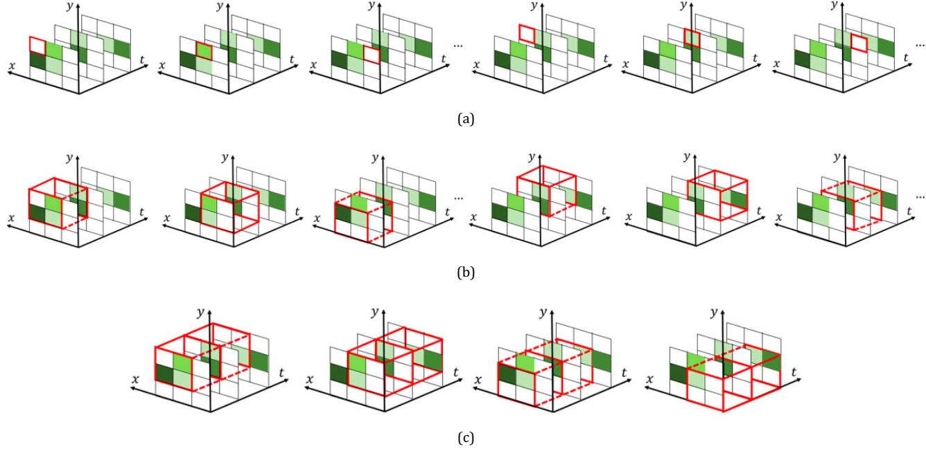
Fig. 5. Illustration of the scanning process with window sizes equal to (a) w = 1 and h = 1 , (b) w = 2 and h = 2 , and (c) w = 2 and h = 3 .
