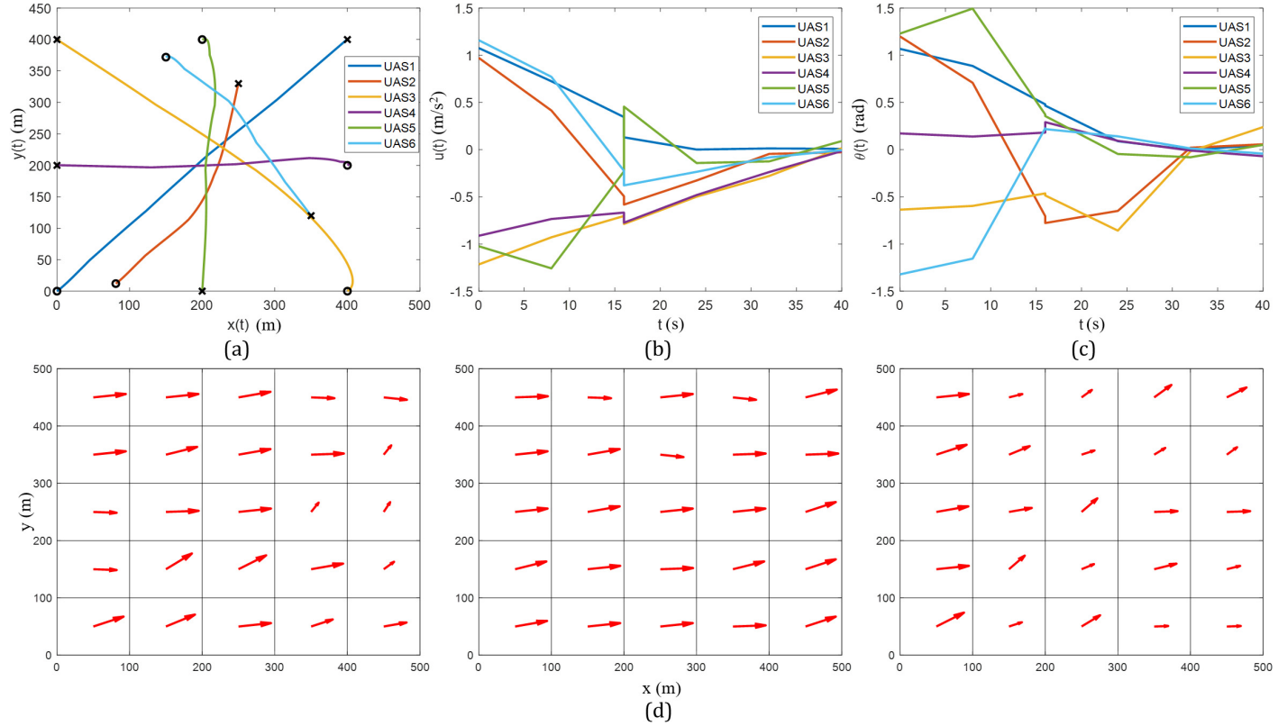
Fig. 11. The optimal 6 UASs trajectory solution for s_{C3} . (a) The trajectories of the 6 UASs. (b) The thrusts. (c) The angles of the thrusts. (d) The sample snapshots of s_{C3} at t = 5 s, t = 22 s, and t = 37 s.
