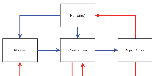
Fig. 1. Co-adaptation template.
