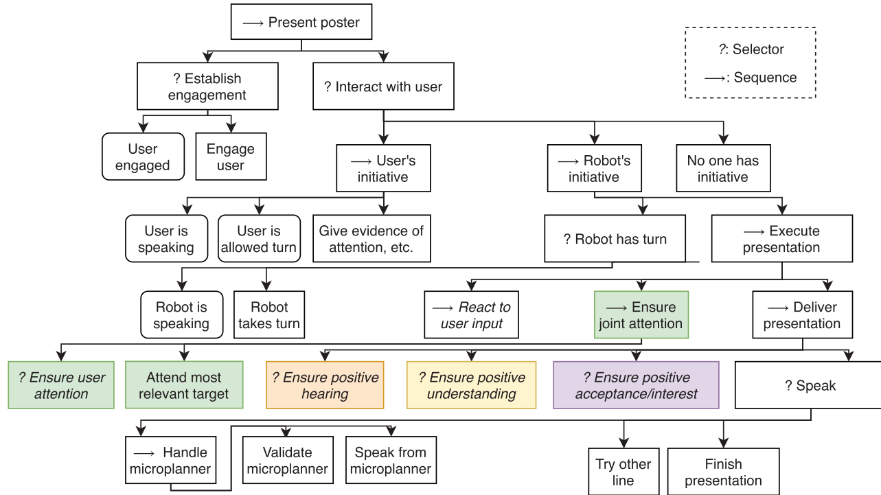
Fig. 7. The behavior tree driving the interactions described in Sec. 5.1. For a brief explanation of the tree, see Sec. 5.1.1. The graphical representation of the tree is adapted from Ref. 61; rounded nodes represent queries and rectangular nodes represent actions . Nodes with text in italics contain sub-trees that were omitted for space; for their implementation, see Ref. 62.
