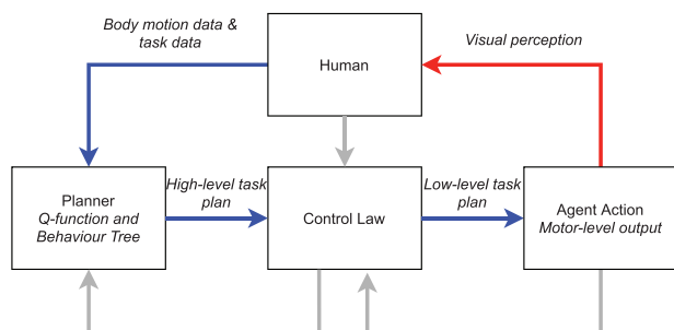
Fig. 8. Co-adaptation for multi-modal interaction (nonverbal).
