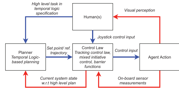
Fig. 2. Co-adaptation for planning and control synthesis.
