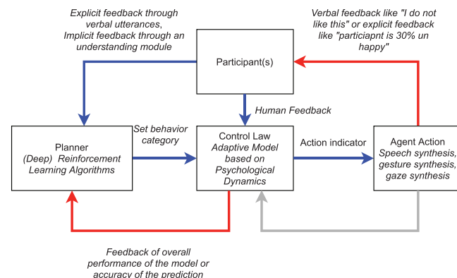
Fig. 3. Co-adaptation for trusted HRIs.
