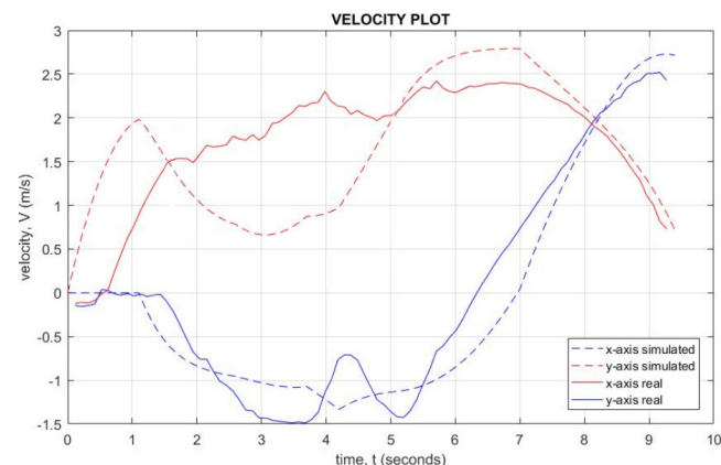
Fig. 12. Velocity profile for the first test set.
