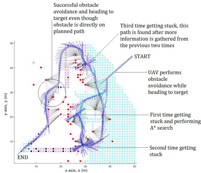
Fig. 11. Exemplary performance of the algorithm demonstrating each component in simulation.
