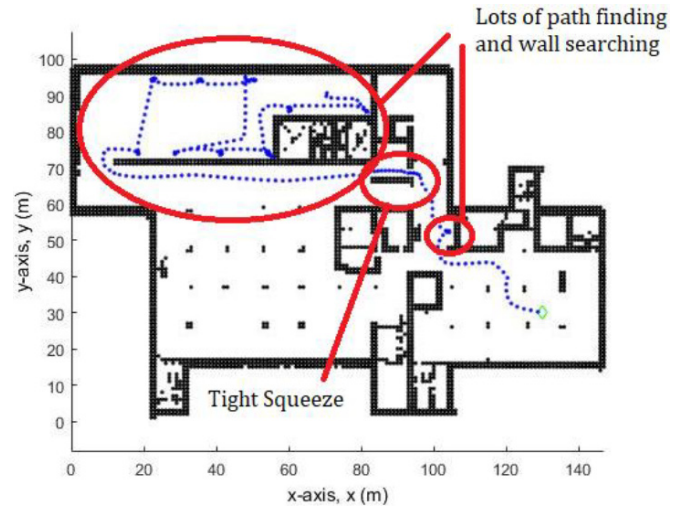
Fig. 19. First run of the UAV in the factory map. A lot of exploration occurs as the UAV tries to learn about its surroundings.
