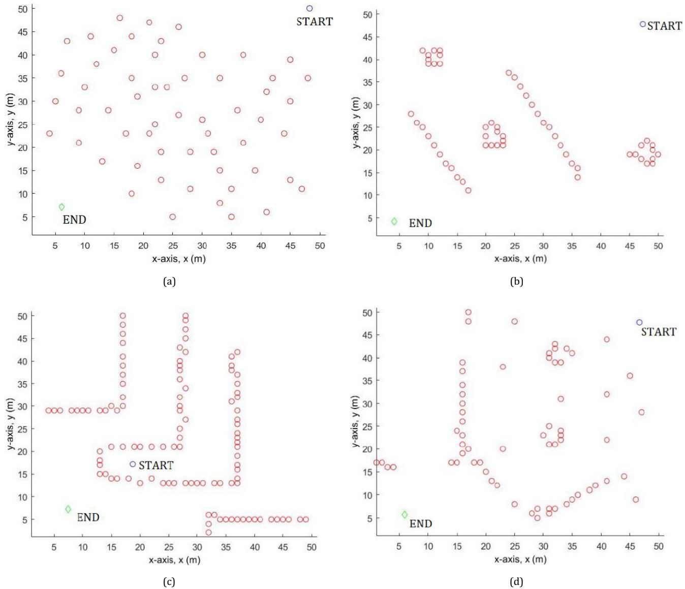
Fig. 17. (a) “Sparse” map space. (b) “Two walls” map space. (c) “Corridor” map space. (d) “Mixed” map space.
