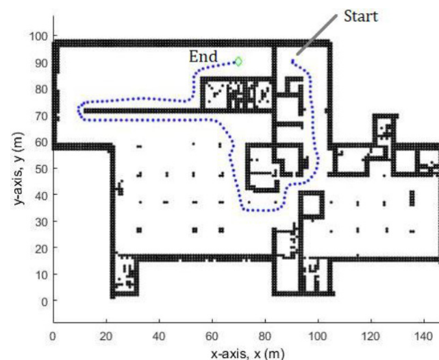
Fig. 22. When the start and end points are changed, smooth performance is the direct result of the algorithm having a more informed local map.
