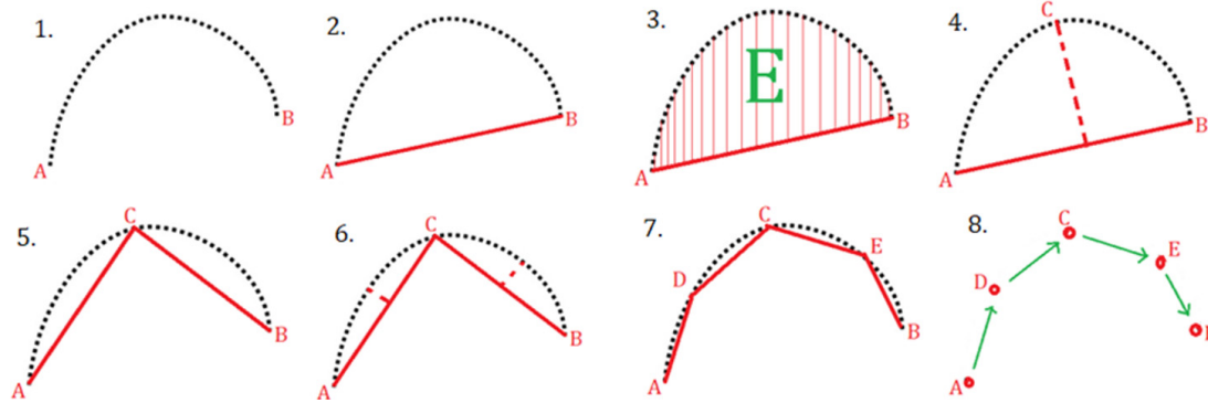
Fig. 9. Split-and-merge algorithm.
