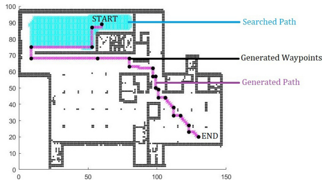
Fig. 10. Split-and-merge algorithm performed on the path generated by the A* algorithm.
