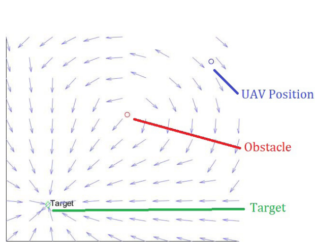
Fig. 7. Vector field formed around each obstacle representing reference velocity heading.
