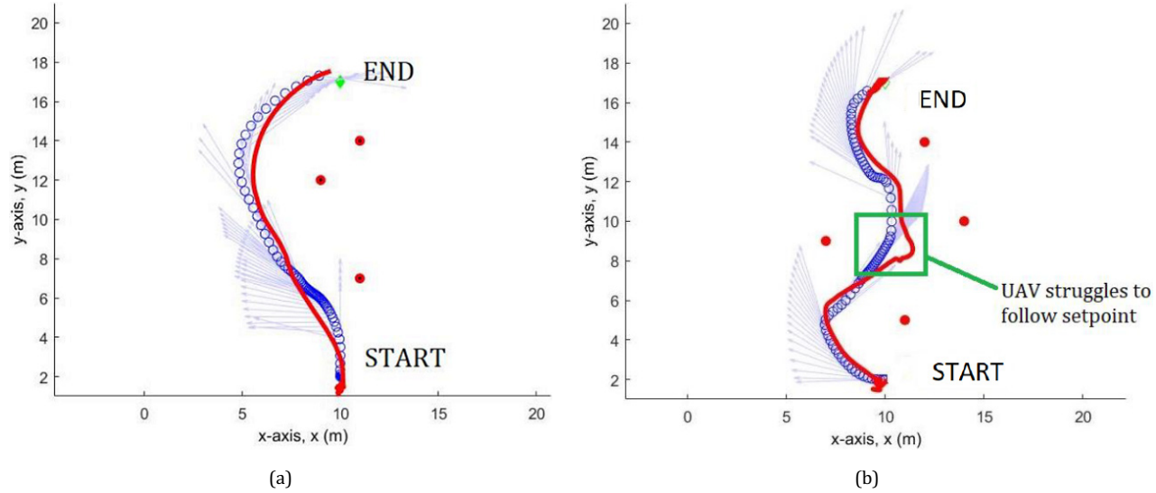
Fig. 15. 2D trajectory for the flight tests against the simulated results. The red line represents the real world UAV trajectory, while the blue circles represent the simulated UAV trajectory. (a) Map 1. (b) Map 2.
