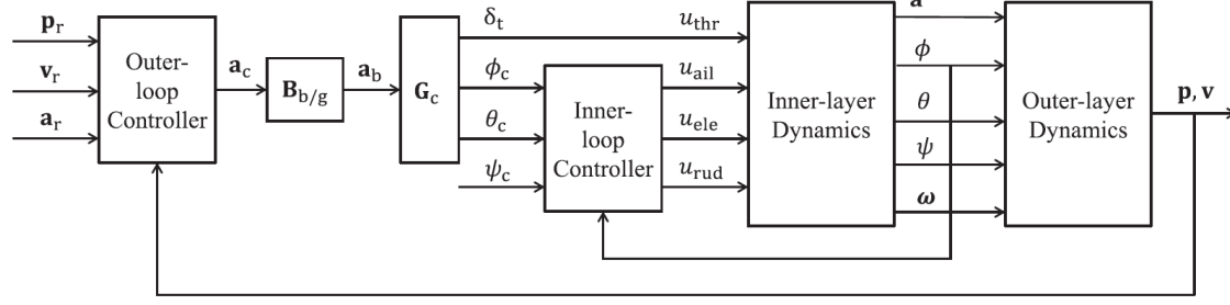
Fig. 3. Two stage control for multirotor UAVs.
