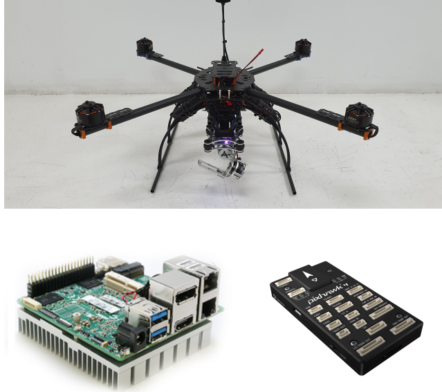
Fig. 1. Top: HLX platform; Bottom Left: Intel UP Squared single board computer; Bottom Right: Pixhawk 4 FMU.
