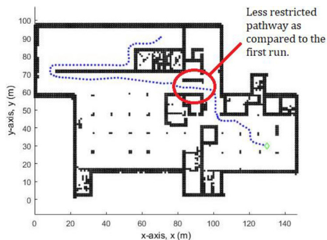
Fig. 20. Second run of the UAV in the factory map. No more exploration is needed as the algorithm figures out the most optimum path right from the get go.
