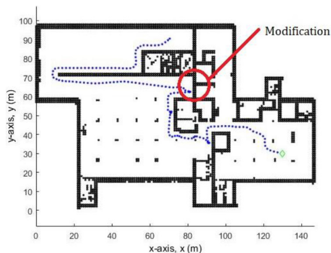
Fig. 21. When the map is changed, the algorithm is able to suitably adapt to find another appropriate path to reach the target.
