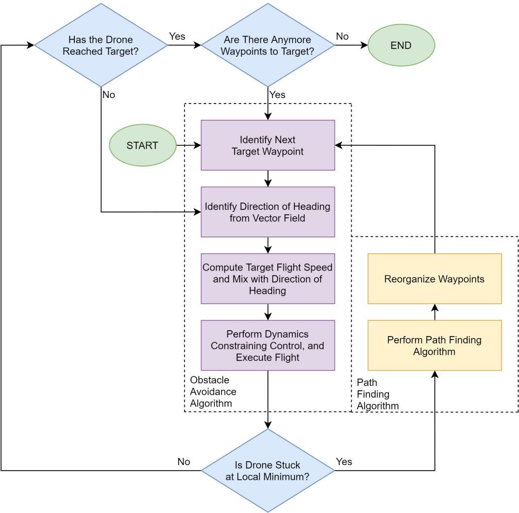
Fig. 6. Overarching algorithm state architecture.
