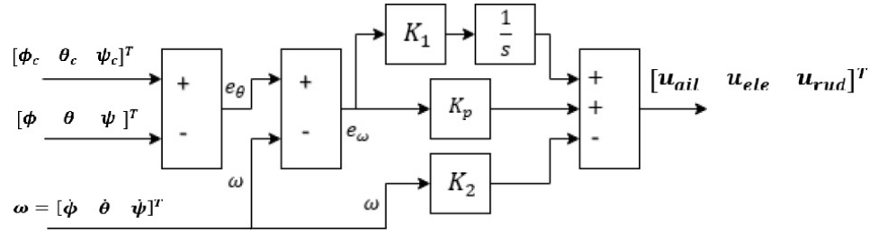
Fig. 4. SIPIC controller used as an inner-loop controller in the UAV.
